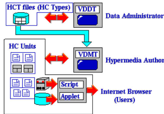
Figure 3: Structure Editor Components
